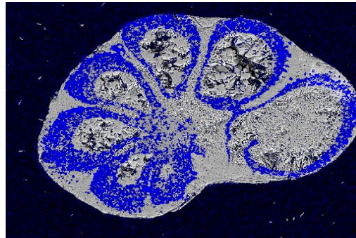
Fig.15. Section of melted foram with calcite-filled chambers.
