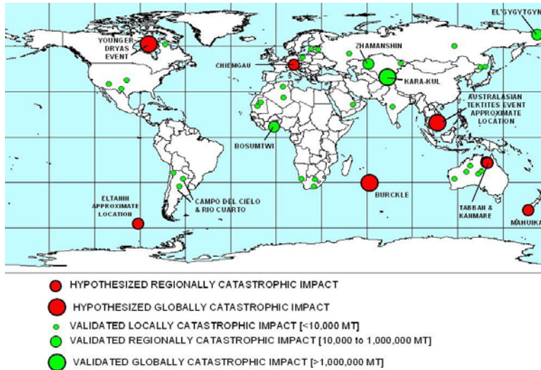
Fig. 3. Validated and selected hypothesized impacts by asteroids and comets during the past five million years.
