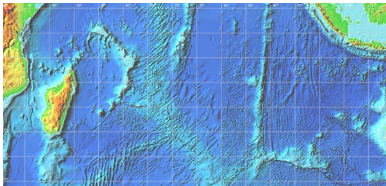
Figure 1. Map of a portion of the Indian Ocean sea floor from on satellite altimetry and transects by oceanic exploration vessels. Longitude 80° east represents the dividing line between higher (east) and lower (west) resolution altimetry [3].
