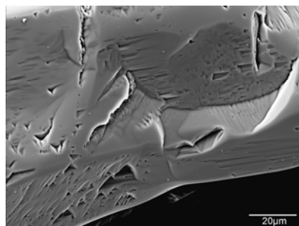
Fig. 12. Micro-grain of shocked quartz exhibiting multiple PDFs.
