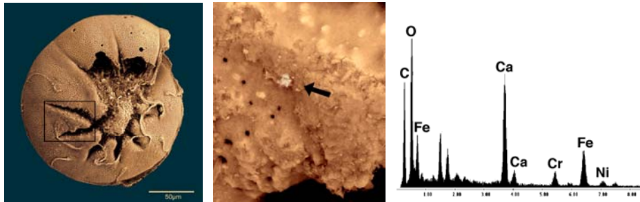
Fig. 14. Unmelted benthonic foram (left) with Fe-Cr-Ni splash (middle), and associated spectrum analysis (right).
