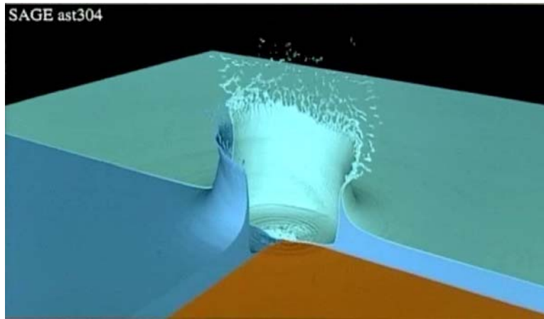
Fig. 2. Three-dimensional model simulation of the splash ring crown of a 1-km diameter oceanic asteroid impact, just prior to the formation of multiple tsunami waves [4].
