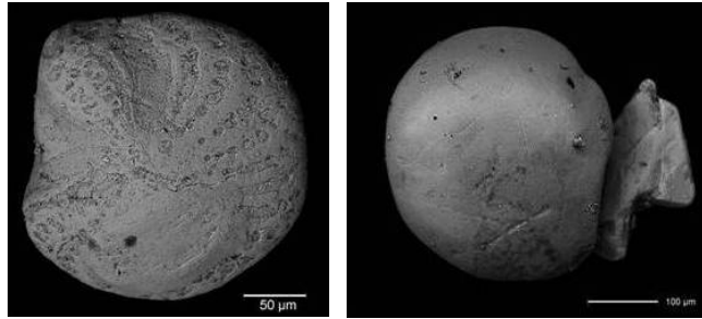
Fig. 13. Melted benthonic foraminifera containing manganese oxide micro-nodules.
