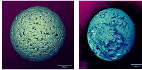
Fig. 8. Impact spherules from upper levels of deep sea cores near Burckle candidate impact structure.
