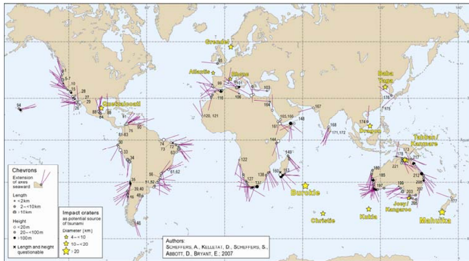
Fig. 4. World map of chevron distribution [15]. The points along the shorelines give only an approximate position due to the scale of the map, and in many cases represent multiple chevrons. The main chevron axes point to possible source areas of tsunamis. Hypothesized oceanic craters are depicted by stars (see also Fig. 3). Figure courtesy of Anja Scheffers.
