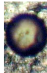
Fig. 11. Translucent graphite.
