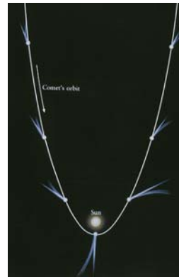
Fig. 20. Orientation of pre- and post-perihelion comet tails.
